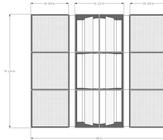
FRONT/BACK VIEW
